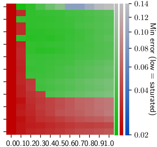
Dataset = Office31
