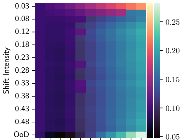
Dataset = Office31
