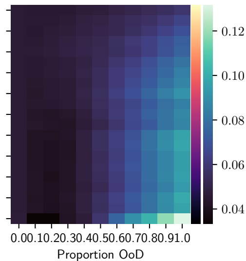
Dataset = OfficeHome
