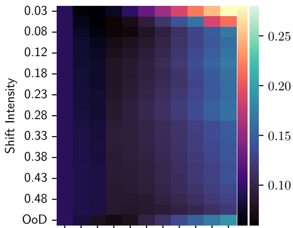
Dataset = CCT
