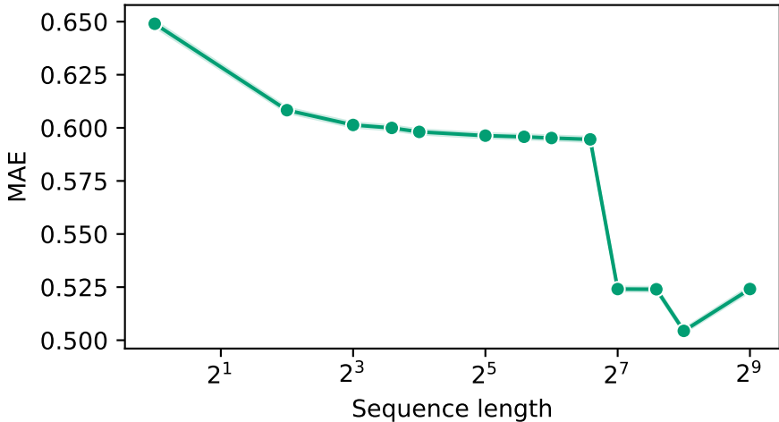
Sequence-length sensitivity
