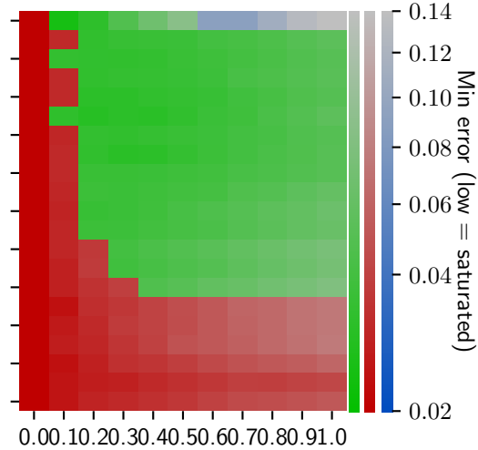
Dataset = Office31
