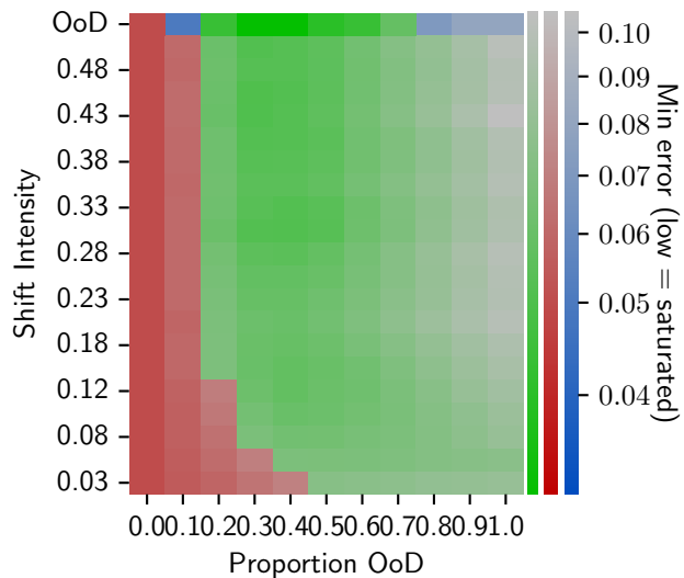
Dataset = OfficeHome
