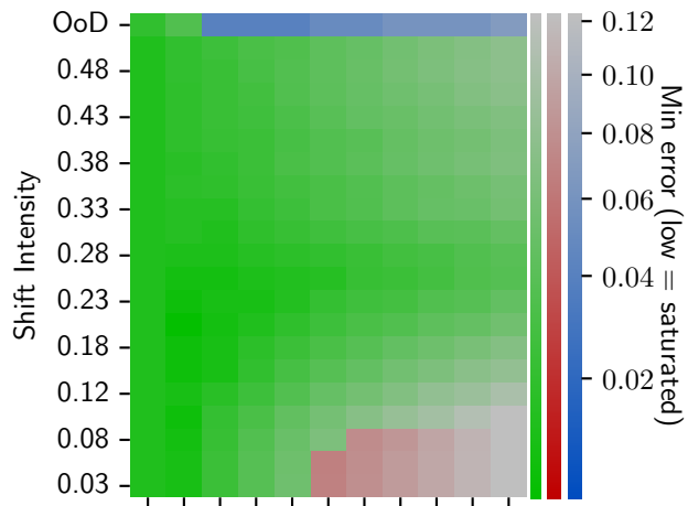
Dataset = CCT
