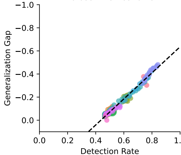
Dataset = OfficeHome
