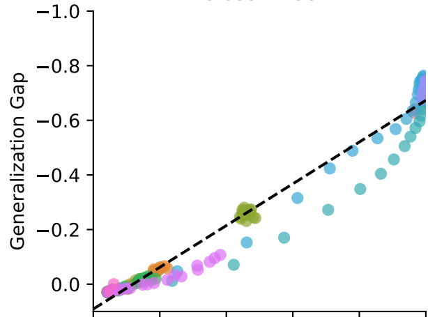
Dataset = CCT
