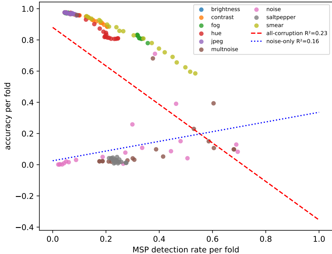
CCT: MSP detection-rate vs accuracy
