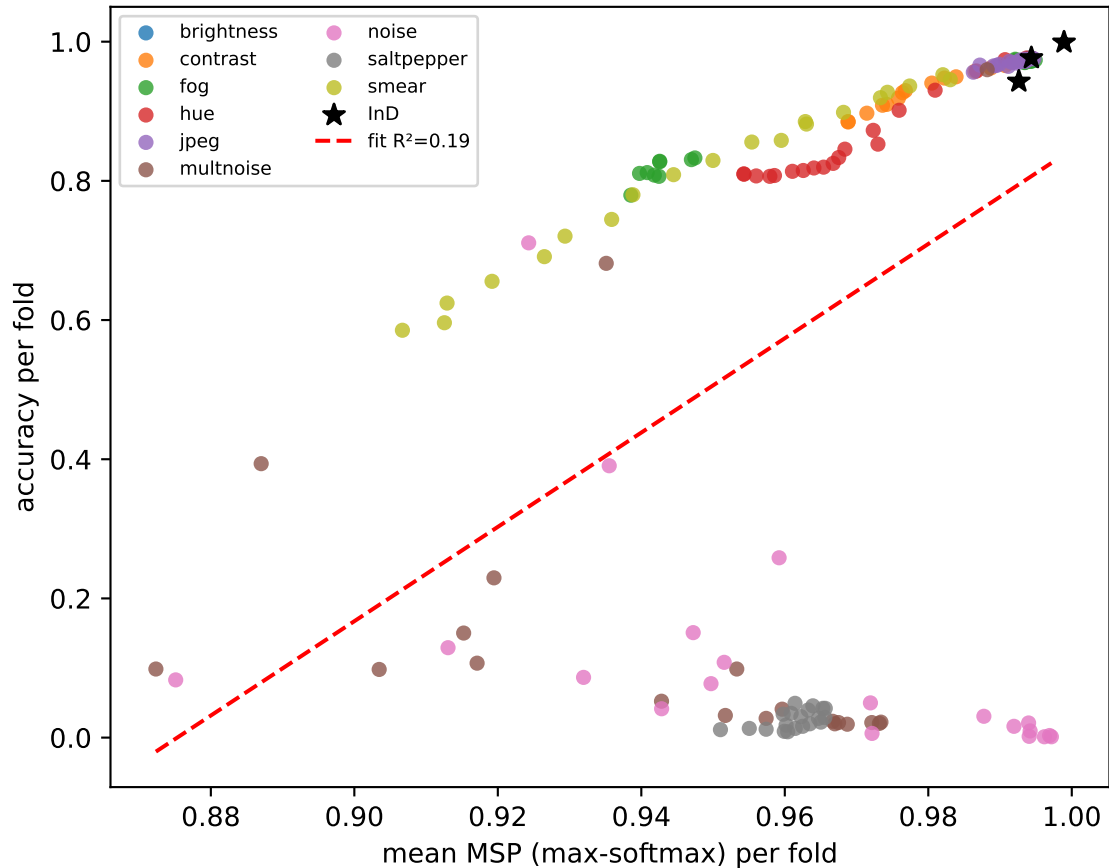
CCT: mean MSP vs accuracy (per synthetic fold)
