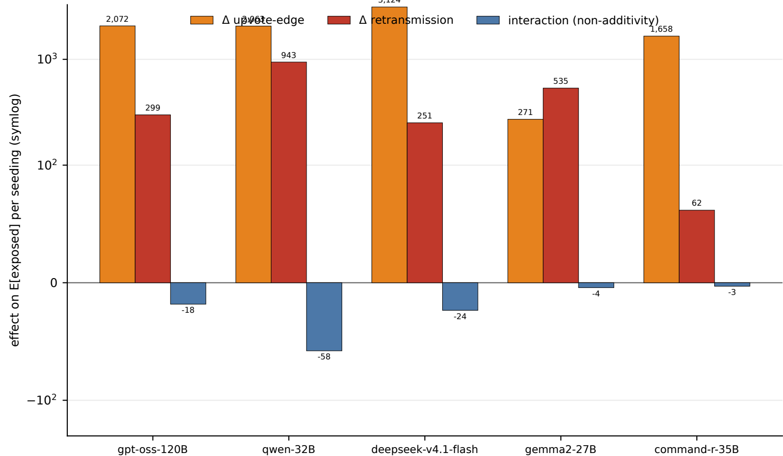
Per-model exposures decomposition
