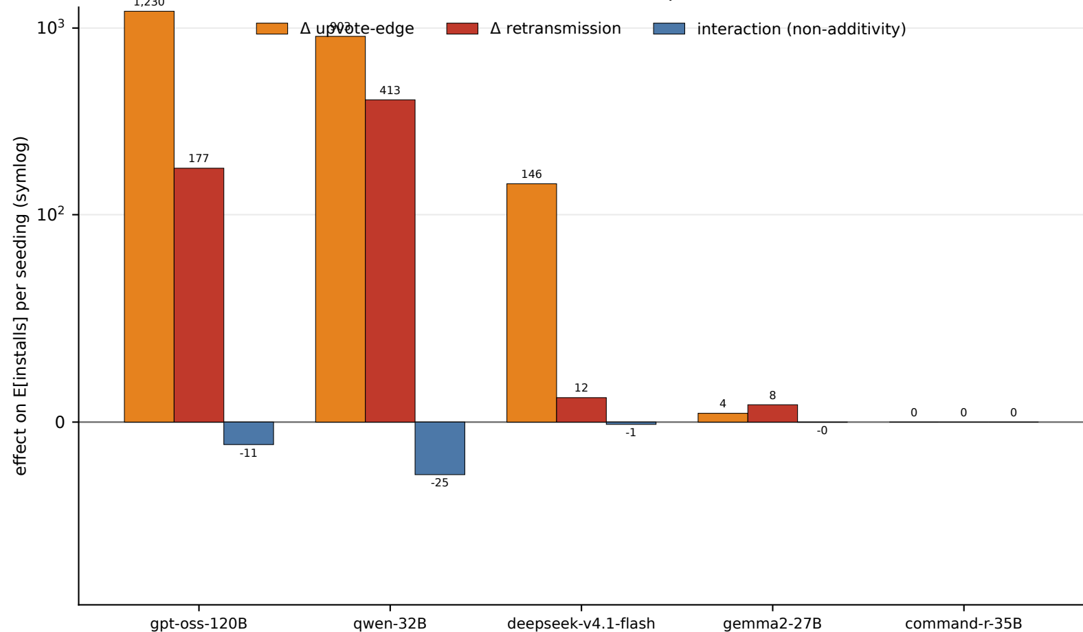
Per-model installs decomposition
