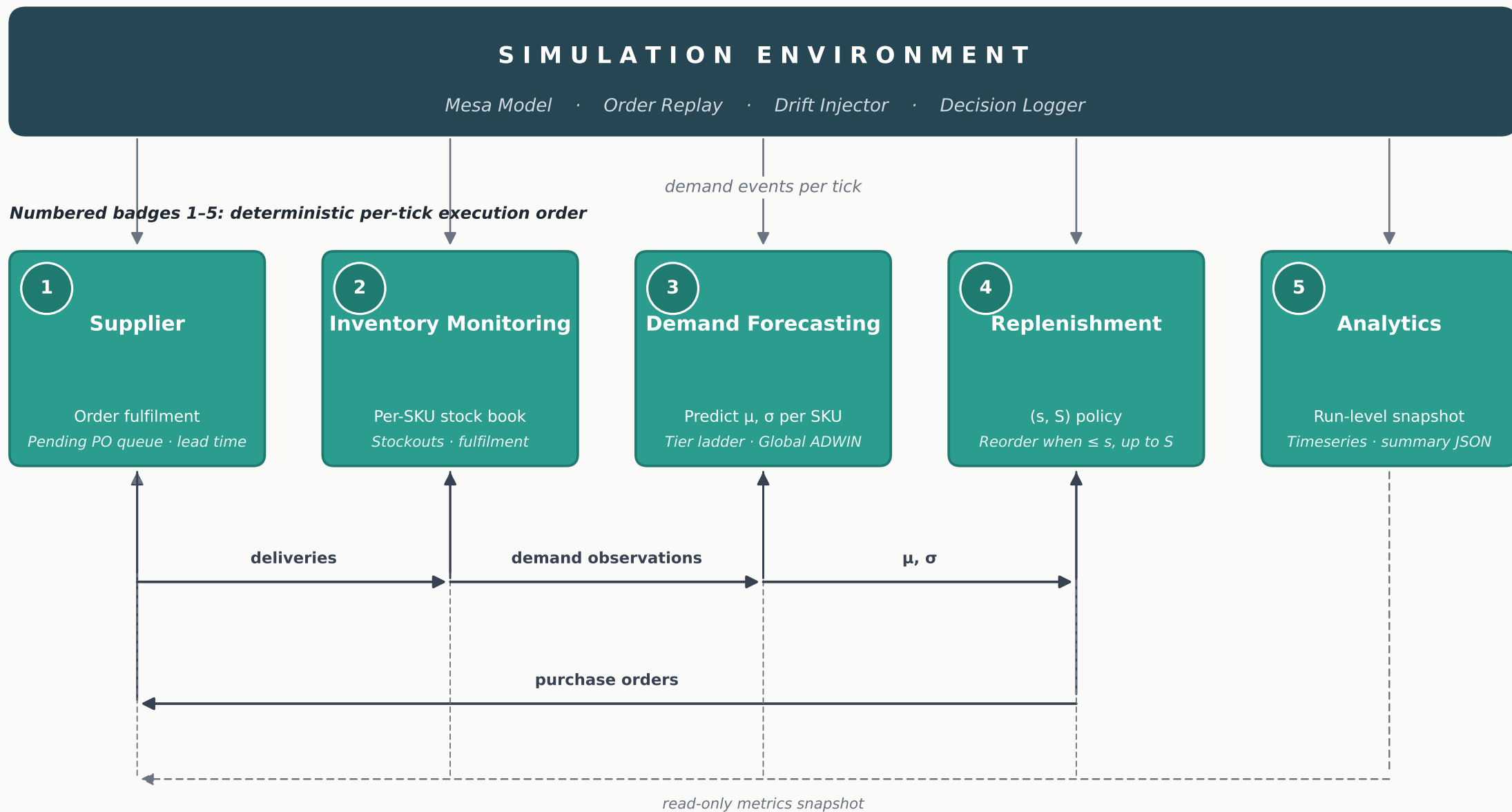
Figure 3.1. High-level architecture. Five autonomous agents are coordinated through a shared Mesa simulation environment. Solid arrows show data flow during one tick; the dashed line is the Analytics agent's read-only observation of post-decision state.
