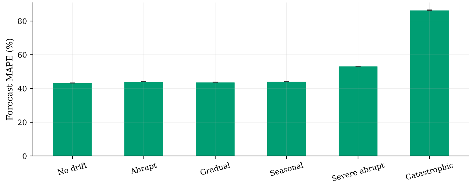
Forecast accuracy under each scenario (MAS, mean across seeds)
