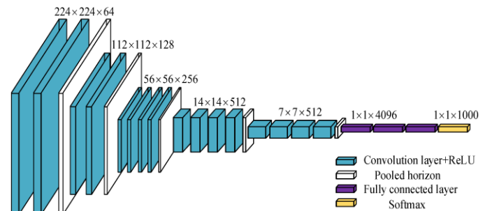
Figure 3. Model Architecture. [12]
