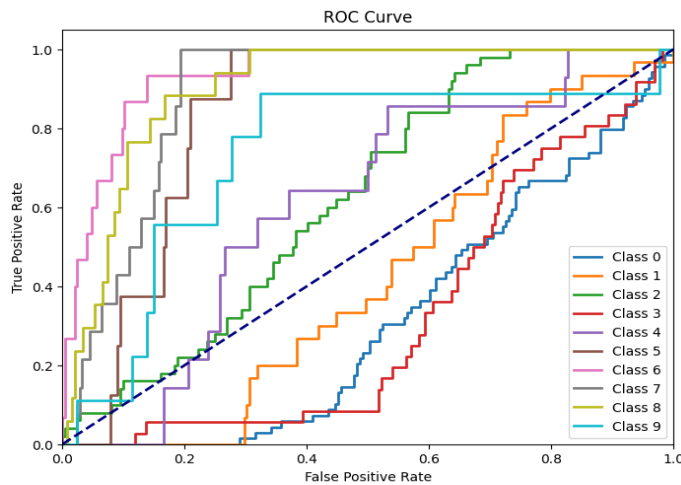
Figure 3. ROC Curve.
