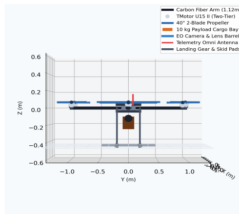
Figure 5.3: Side elevation view showcasing the 450 mm landing gear height, providing a 220 mm ground clearance buffer to protect the camera gimbal.
