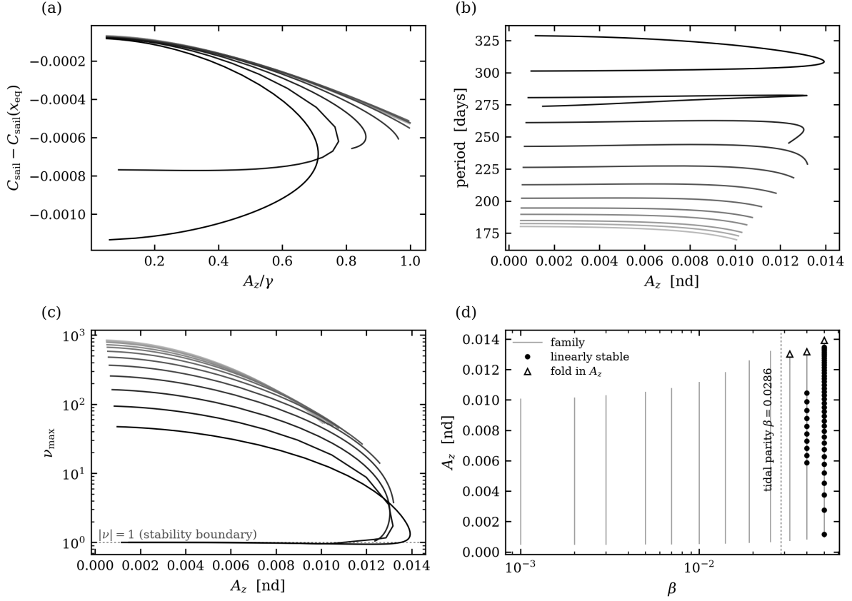
Figure 4: Halo families across \beta \in [0.001, 0.05] , Sun--Earth, \alpha = 0 , walked by pseudo-arclength continuation with branch identity enforced across \beta . (a) Family depth below the local equilibrium in the sail potential, against amplitude scaled by the local length \gamma . (b) Period. (c) Stability index, with the |\nu| = 1 boundary. (d) The (\beta, A_z) plane: family extent, folds, and linearly stable segments, with tidal parity marked.
