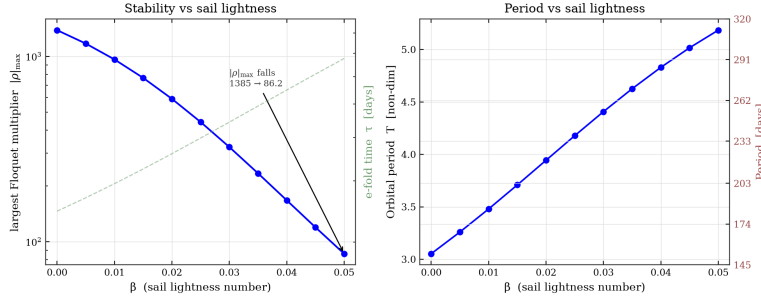
Fig. 5 Largest Floquet multiplier (left) and period (right) of the L_1 halo orbit with A_z = 0.003 across the flown band 0 \leq \beta \leq 0.05 ; every member is checked to be a halo rather than a vertical Lyapunov orbit. The decline is not sail stabilisation of a saddle: the standoff grows, the smaller primary’s tidal term weakens, and the orbit moves away from the saddle it began near.
