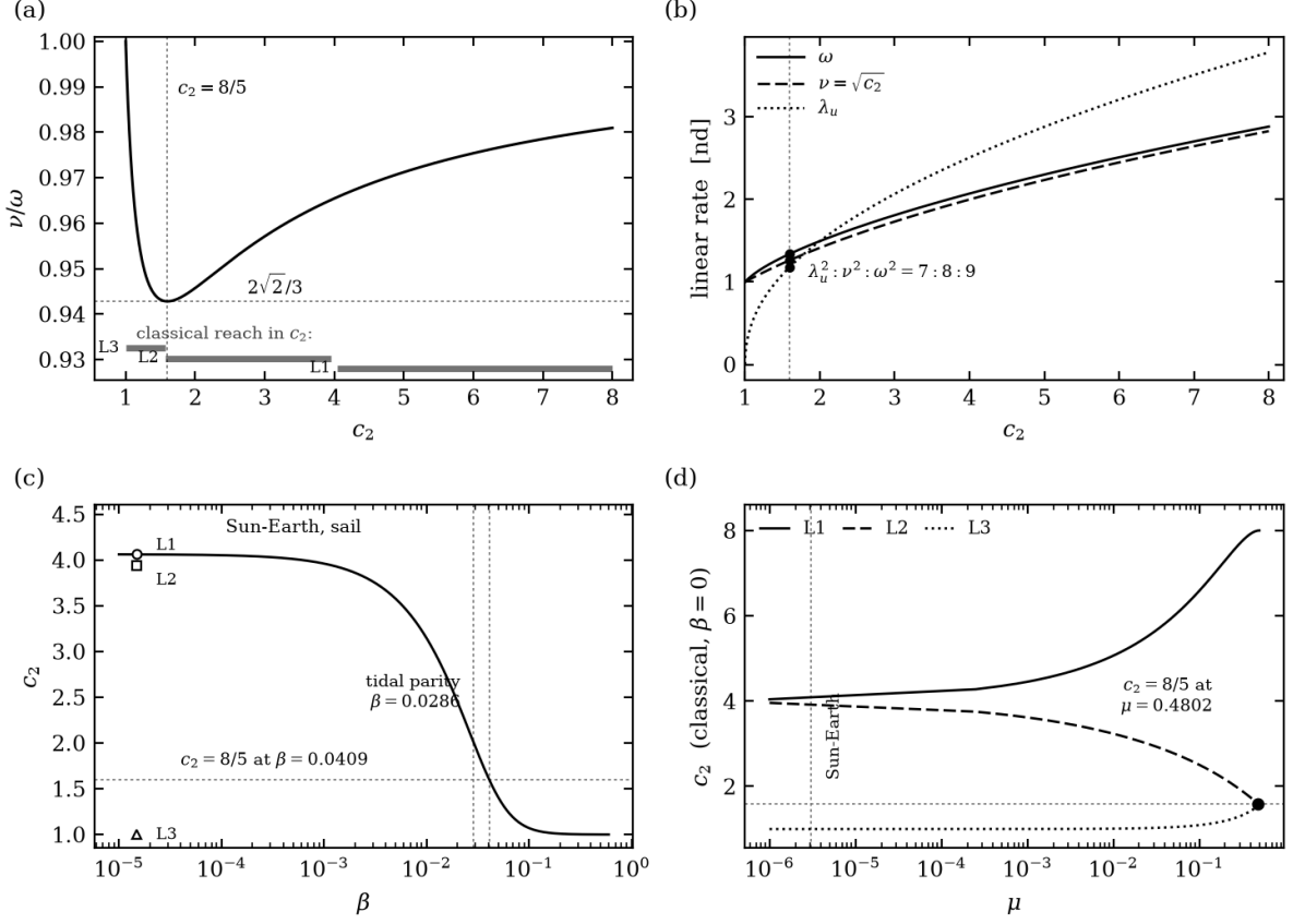
Figure 3: The frequency ratio at collinear equilibria. (a) \nu/\omega against c_2 , with the exact minimum 2\sqrt{2}/3 at c_2 = 8/5 and, in the reserved strip below, the ranges of c_2 reached by the three classical collinear points over \mu \in (0, \frac{1}{2}] ; the vertical placement of those bars is a layout choice and carries no value. (b) The three linear rates, meeting the ratio 7 : 8 : 9 at c_2^* . (c) The sail’s tuning curve for Sun–Earth: c_2(\beta) sweeps continuously from the classical value down to unity, passing tidal parity and then c_2^* . Open markers give the three classical Sun–Earth values, none of which is at the bound. (d) Classical c_2 against \mu for all three points; c_2^* is attained at L_2 for \mu = 0.4802 .
