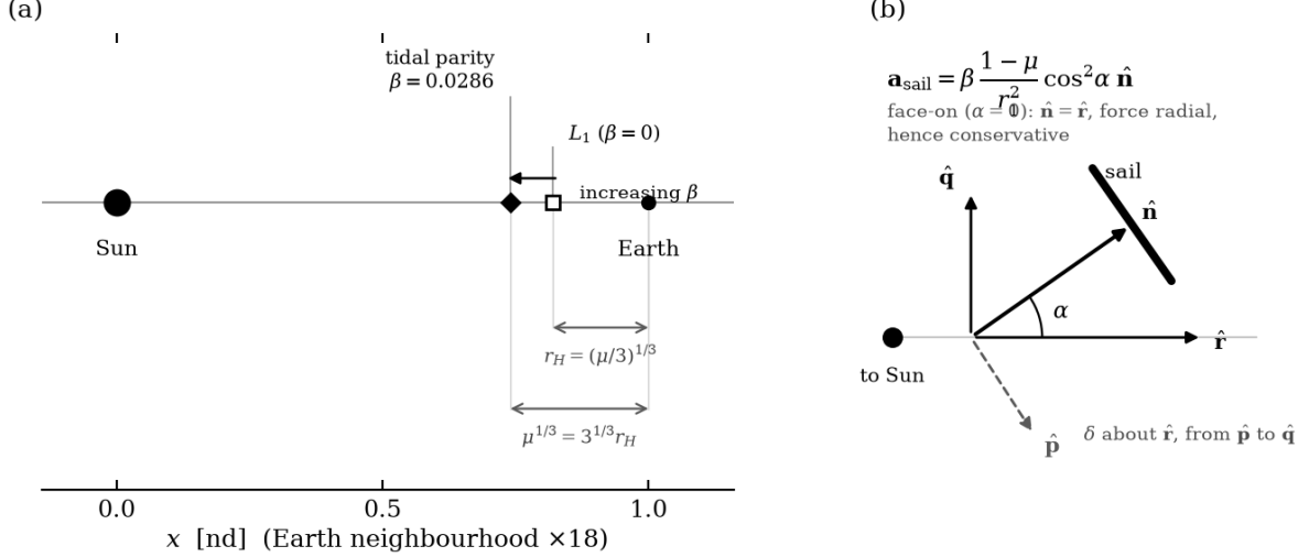
Figure 1: Geometry of the face-on solar-sail CR3BP. (a) The synodic frame. The classical L_1 lies essentially on the Hill sphere ( r_2 = 0.9967 r_H ); as \beta grows the equilibrium migrates sunward, reaching the tidal-parity radius r_2 = \mu^{1/3} = 3^{1/3} r_H at \beta = 0.0286 . The Earth neighbourhood is exaggerated by a factor of 18; at true scale every feature would collapse onto the smaller primary. (b) Attitude convention and the orthonormal triad (4). At \alpha = 0 the normal is \hat{r} , the force is radial, and the sail is conservative.
