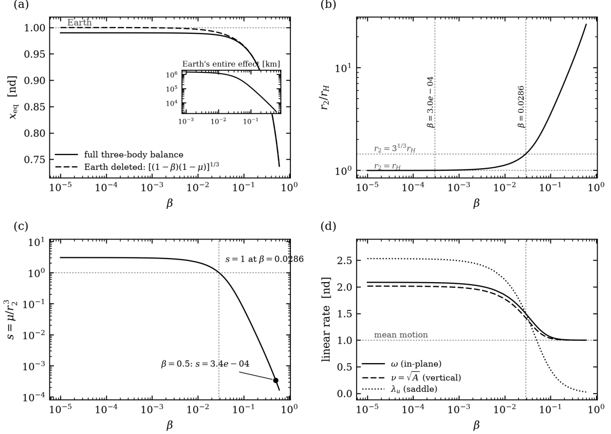
Figure 2: Dissolution of the Sun–Earth collinear structure. (a) The full three-body equilibrium is indistinguishable from the Earth-free hovering law (7); the inset shows the smaller primary’s entire contribution collapsing to a few thousand kilometres. (b) The standoff crosses the Hill sphere almost immediately (at \beta = 2.98 \times 10^{-4} , the Hill-exit value, not \beta_{\text{crit}} ) and reaches 20.6 r_H by \beta = 0.5 . (c) The saddle strength falls four decades; s = 1 locates tidal parity. (d) Both frequencies converge on the mean motion and \lambda_u \rightarrow 0 : the Keplerian epicyclic degeneracy of an inverse square field, not a resonance with the smaller primary.
