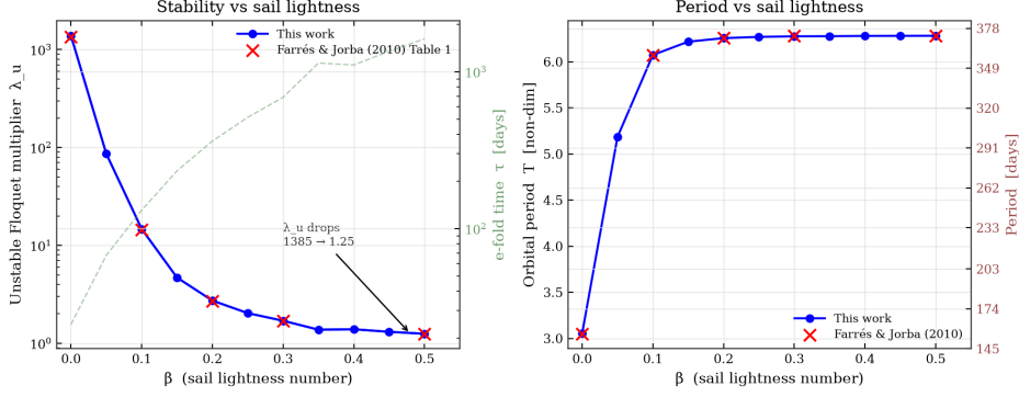
Figure 5: Collapse of the unstable eigenvalue with \beta . The trend is not sail stabilisation of a saddle: the standoff grows, the smaller primary’s tidal term dies, and the orbit moves away from the saddle it began near.
