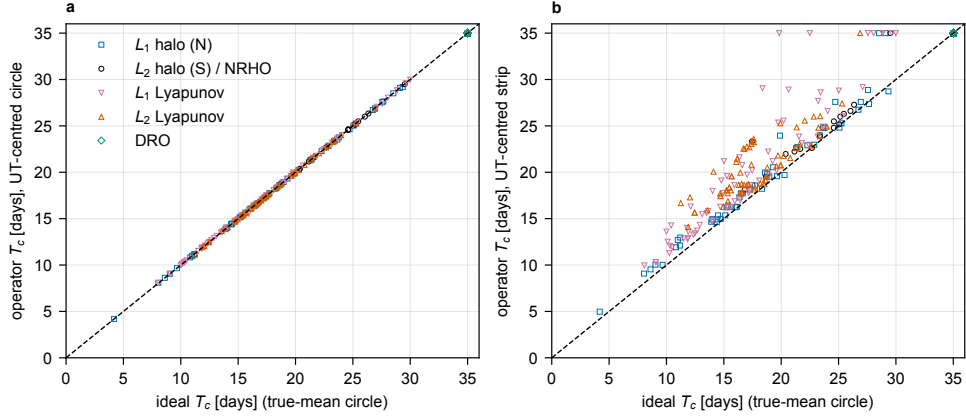
Fig. 15 Operator against ideal custody horizon (ten fields) for the 413 family-sweep cases: a circle centred on the UT prediction, b strip along the UT-predicted sky ellipse. Horizons beyond 30 d are plotted at 35 d; the dashed line is equality
