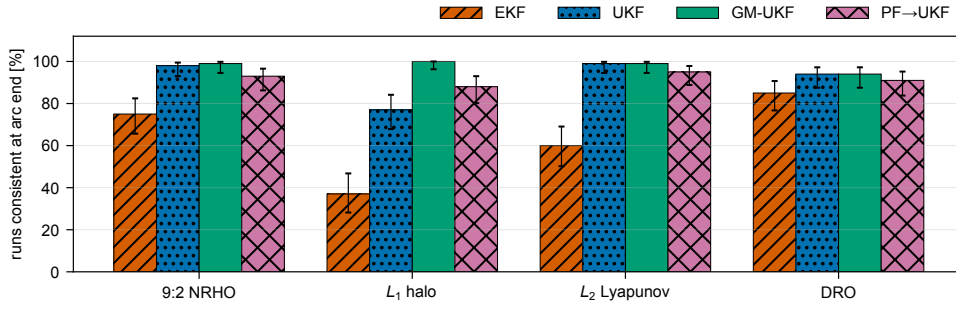
Fig. 7 Share of reacquisition runs ending consistent, by filter and orbit (100 runs each; initial gaps of 1.9–3.2 d); error bars are 95 % Wilson intervals
