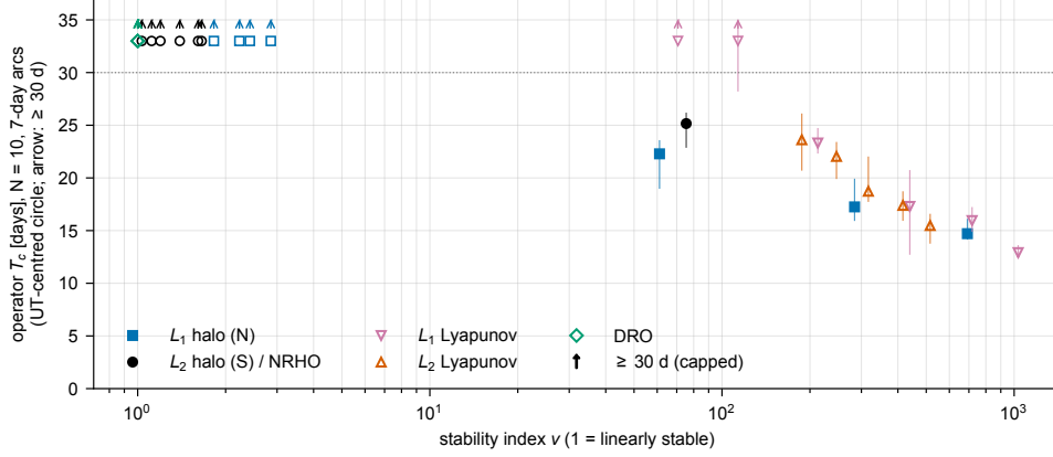
Fig. 14 Operator custody horizon (UT-centred circle, ten fields, 7-day arcs) against the stability index \nu for 30 members of five families: median over arcs (markers) and 10–90 % range over arcs (vertical lines). Members whose median exceeds 30 d are drawn above the dotted line with an arrow. Open markers: Lyapunov families and members beyond 30 d
