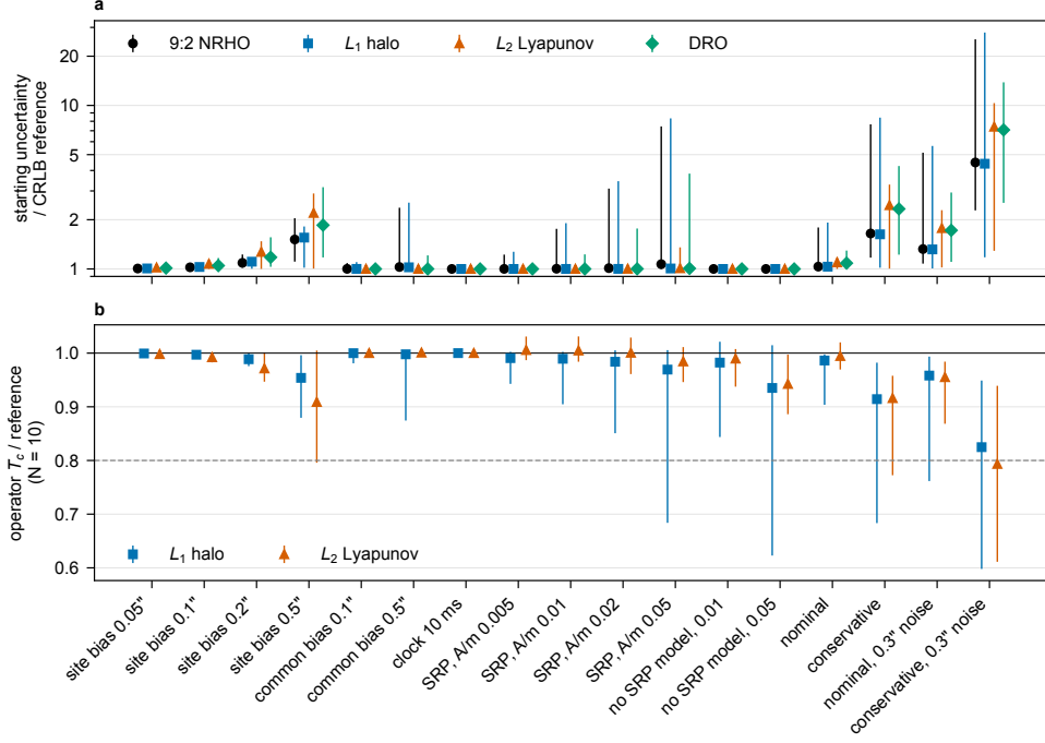
Fig. 16 Effect of unmodelled errors on custody: a starting uncertainty relative to the Cramér–Rao reference (largest 1\sigma position axis), b operator horizon (ten fields) relative to the reference for the arcs whose reference horizon is below 30 d. Markers are medians and lines 10–90 % ranges. Configurations: per-site bias, common bias, clock offset, solar radiation pressure modelled with A/m uncertain by 30 %, solar radiation pressure not modelled, and the nominal and conservative combinations, the last two also with 0.3'' white noise (reference: the 0.3'' Cramér–Rao bound). An unmodelled force shifts the mean rather than widening the covariance, so its value in a is 1. The dashed line marks a 20 % loss
