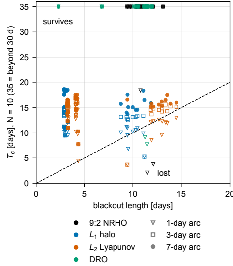
Fig. 9 Ideal custody horizon (ten fields; the operator horizon differs by at most 0.8 d) against blackout length. Points above the diagonal survive the blackout; marker shape shows the tracking-arc length (open: 1 and 3 days, filled: 7 days)
