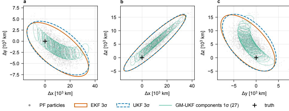
Fig. 6 L_1 halo: predicted uncertainty at the first measurement after the 3.0-day initial gap (run 0), relative to the truth, in the a xy , b xz and c yz synodic planes. Grey dots are PF particles; EKF and UKF 3\sigma ellipses and GM-UKF components ( 1\sigma ) are shown
