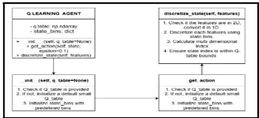
Figure 2: Diagram of QLearningAgent Class
