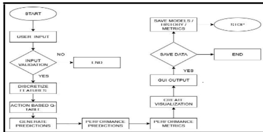
Figure 1: Flow Chart of Data Processed By Q-Learning Agent Functionality
