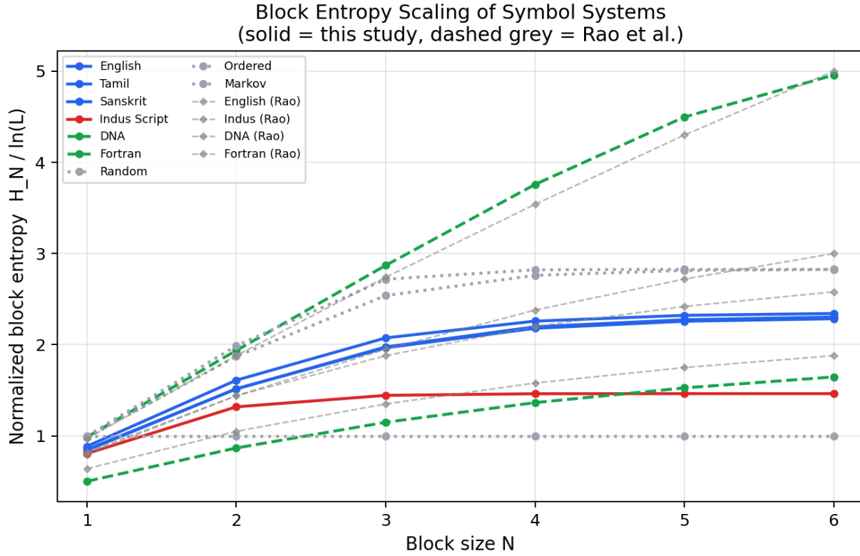
Figure 1. Normalized block entropy H_N / \ln(L) vs block size N . Solid: this study. Dashed grey: Rao et al. published values. Linguistic systems (blue) and the Indus script (red) cluster together. DNA (green dashed) is higher; Fortran lower.
