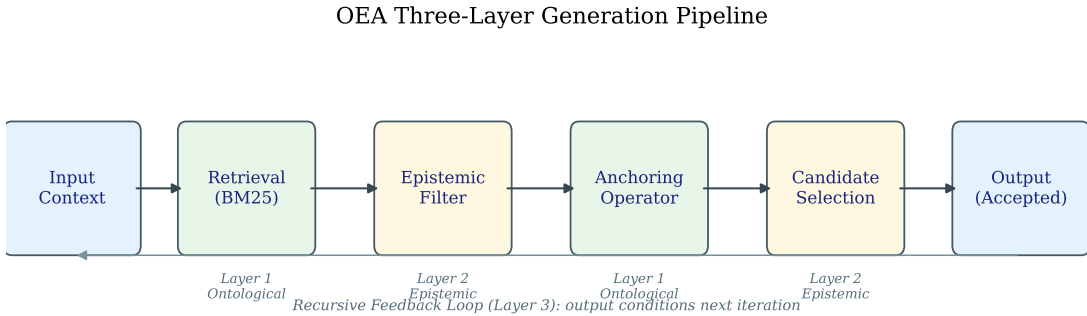
Figure 1: Operational OEA generation pipeline. Retrieval supplies context, the epistemic filter rejects low-quality candidates, anchoring constrains recursive propagation, and the recursive feedback loop conditions the next iteration. The diagram describes substrate-level recursive control, not autonomous agency.
