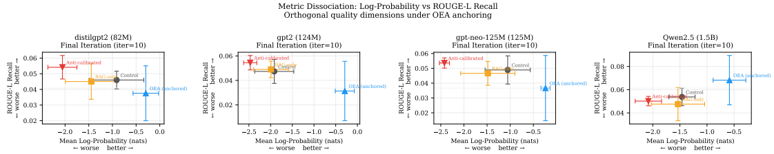
Figure 3: Metric dissociation at final iteration (mean \pm 95% CI, 10 seeds). Log-probability and ROUGE-L capture orthogonal quality dimensions: oea_anchored achieves high log-probability but reduced ROUGE-L (expected under vocabulary anchoring); the inverse holds for oea_miscalibrated . This systematic dissociation addresses metric-circularity concerns.
