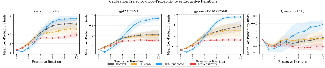
Figure 2: Calibration trajectories across four language models (82M–1.5B). Higher mean log-probability indicates greater distributional fidelity under the frozen evaluator. OEA anchoring improves final-iteration log-probability across all tested models, while the anti-calibrated condition consistently degrades, providing directional ablation evidence for calibration direction. Qwen2.5-1.5B (2024 architecture) extends the validation beyond GPT-2-family models.
