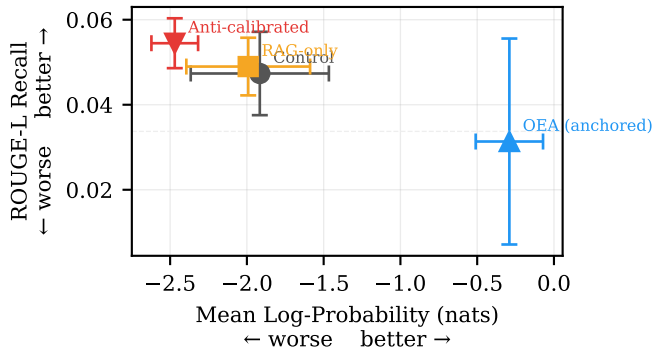
gpt2 (124M) Final Iteration (iter=10)
