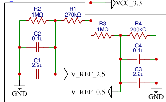
V_REF GENERATION
