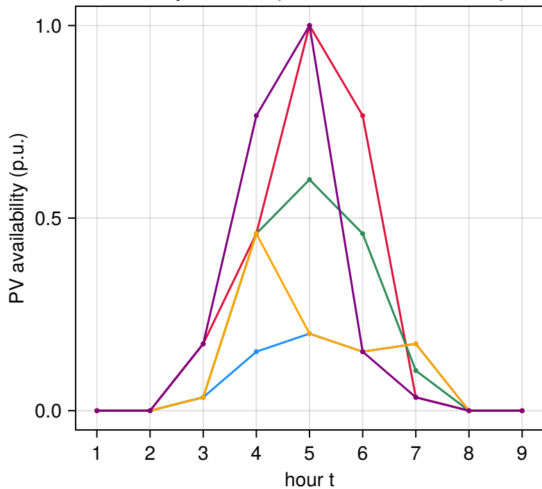
In-sample PV fan (5 seeded Markov draws)
