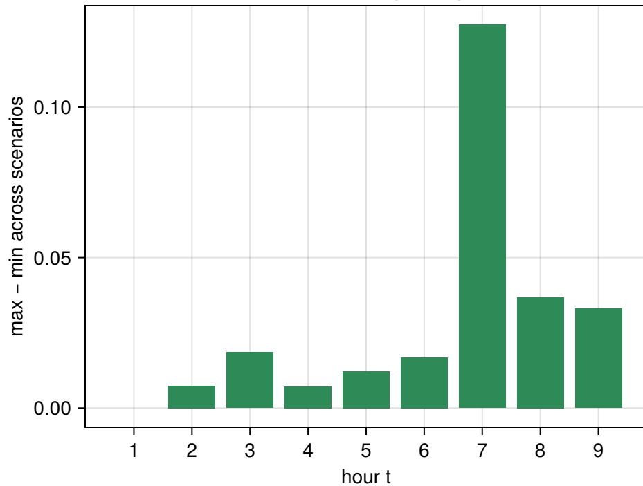
Per-hour scenario price spread
