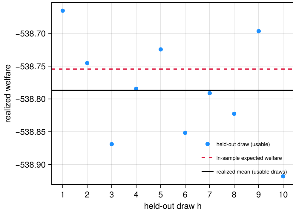
Committed schedule vs 10 unseen futures (gap = -0.0324, 0 infeasible, 0 inexact)
