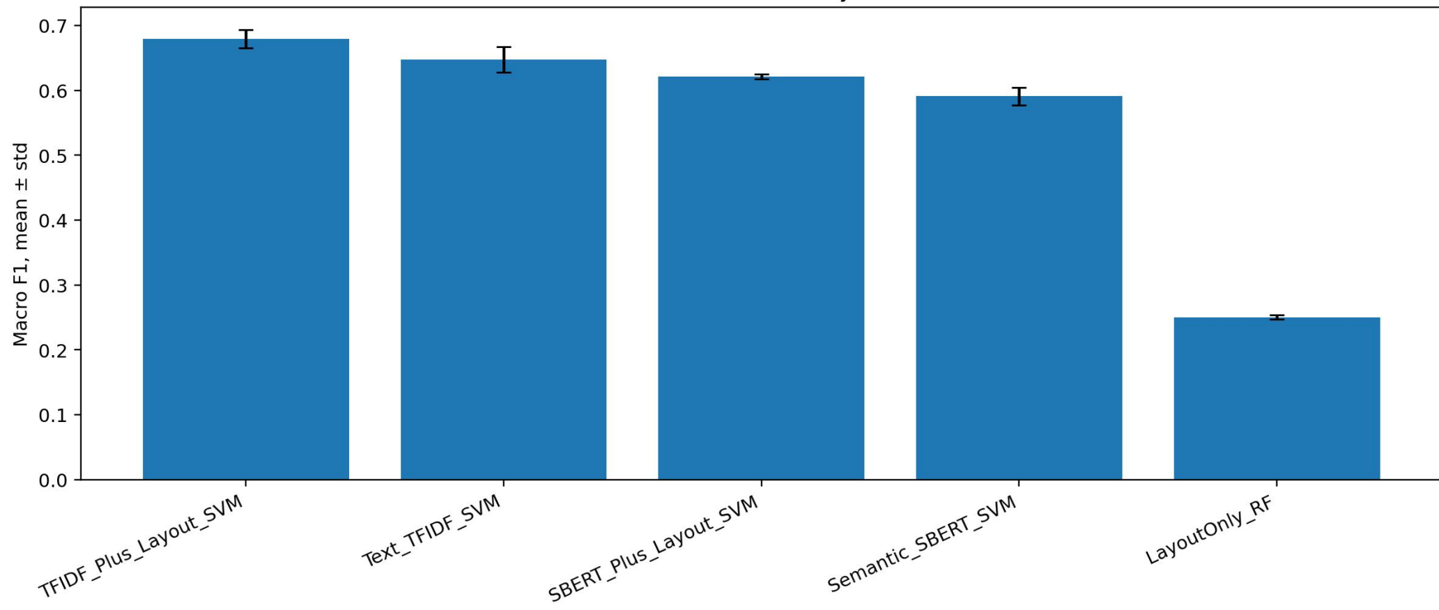
RQ2: Text vs Semantic vs Layout vs Fusion
