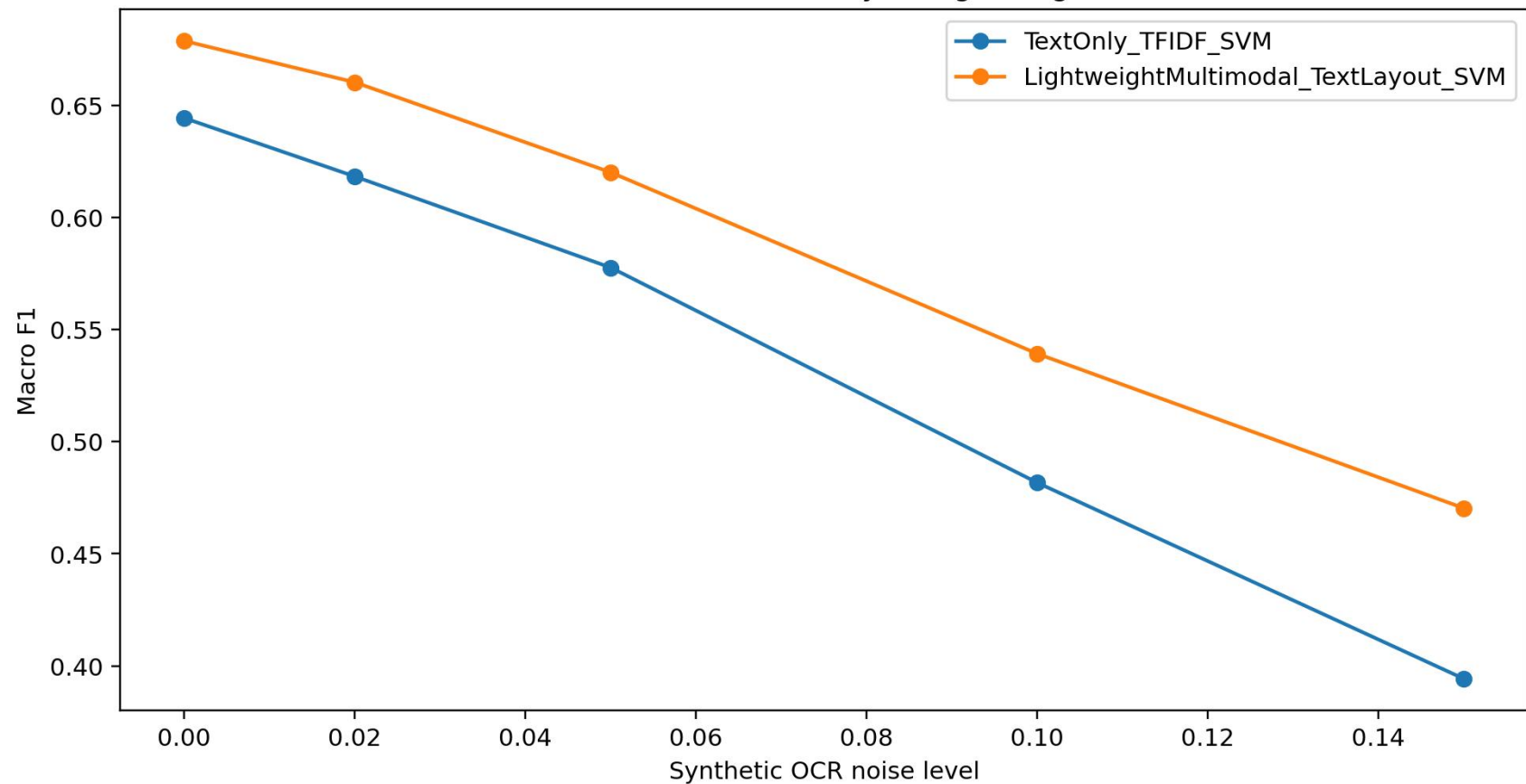
RQ4: OCR Robustness of Text-Only vs Lightweight Multimodal
