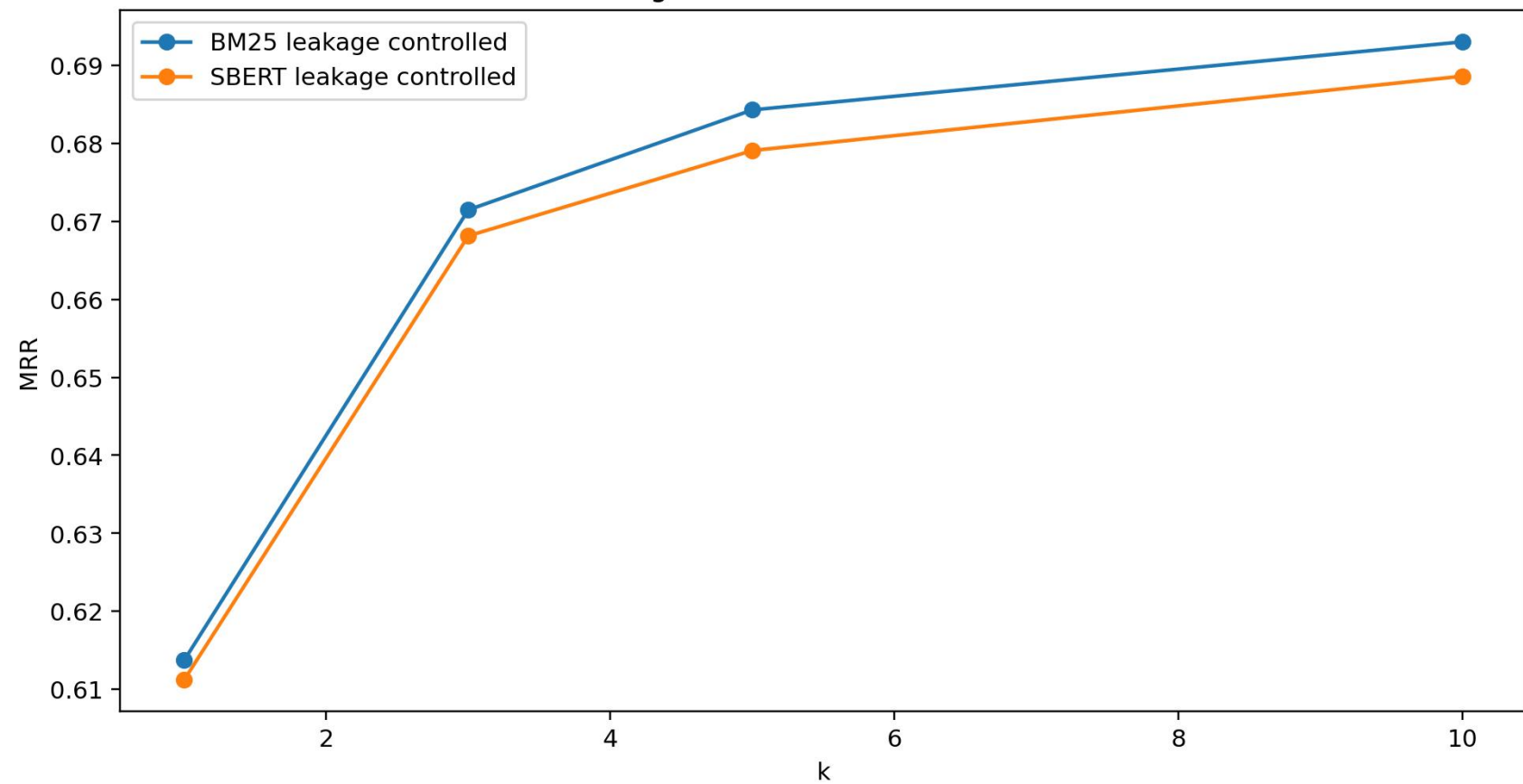
RQ5: Leakage-Controlled Clause Retrieval MRR
