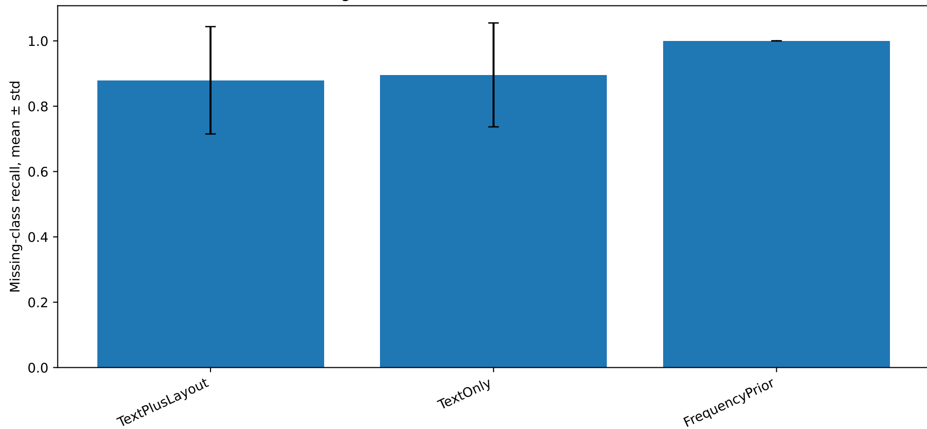
RQ3: Missing-Clause Recall under Validation-Tuned Thresholds
