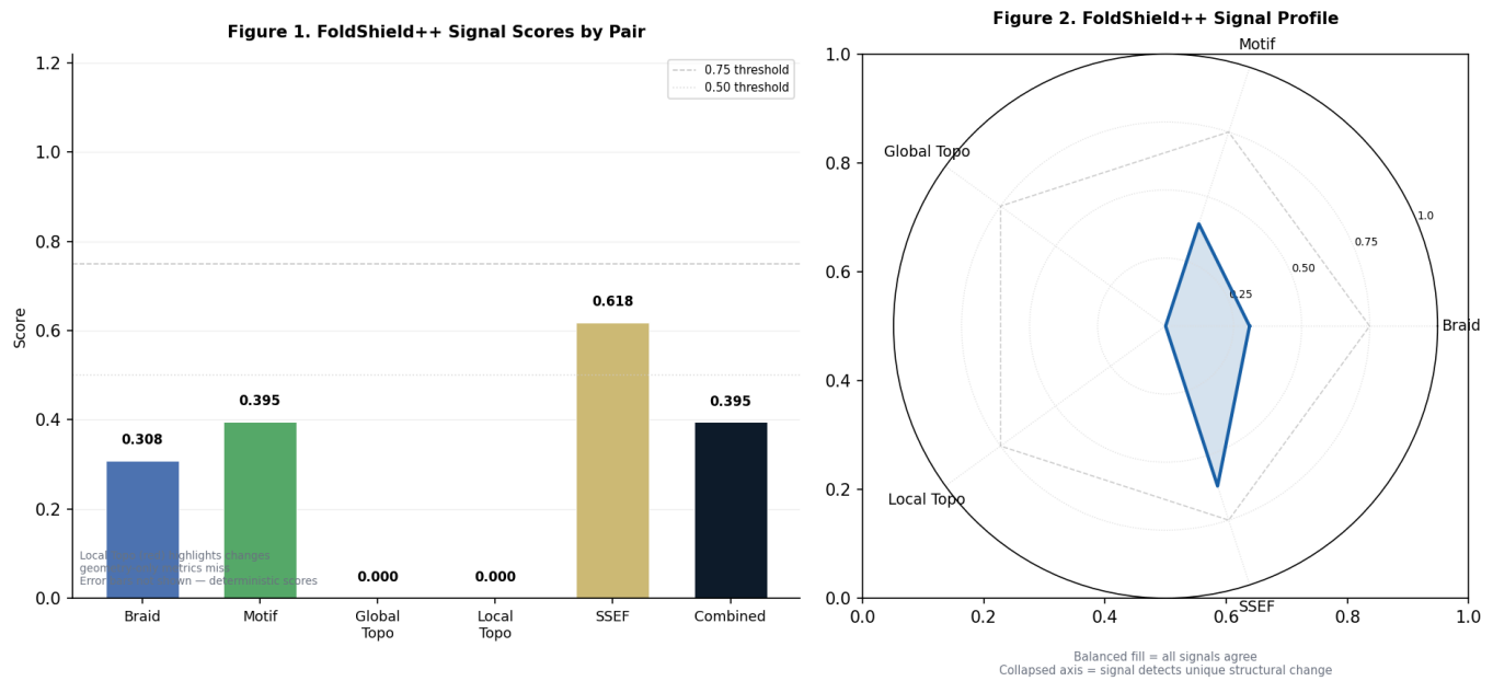
Figure 1: Bar chart comparing all five signals and the Combined score. Local Topo (red) highlights structural changes geometry-only metrics miss. Dashed = 0.75 · Dotted = 0.50. Error bars not shown — scores are deterministic. Figure 2: Radar chart showing the five-signal profile. Balanced fill = all signals agree. Collapsed axis = signal detects unique structural change.
