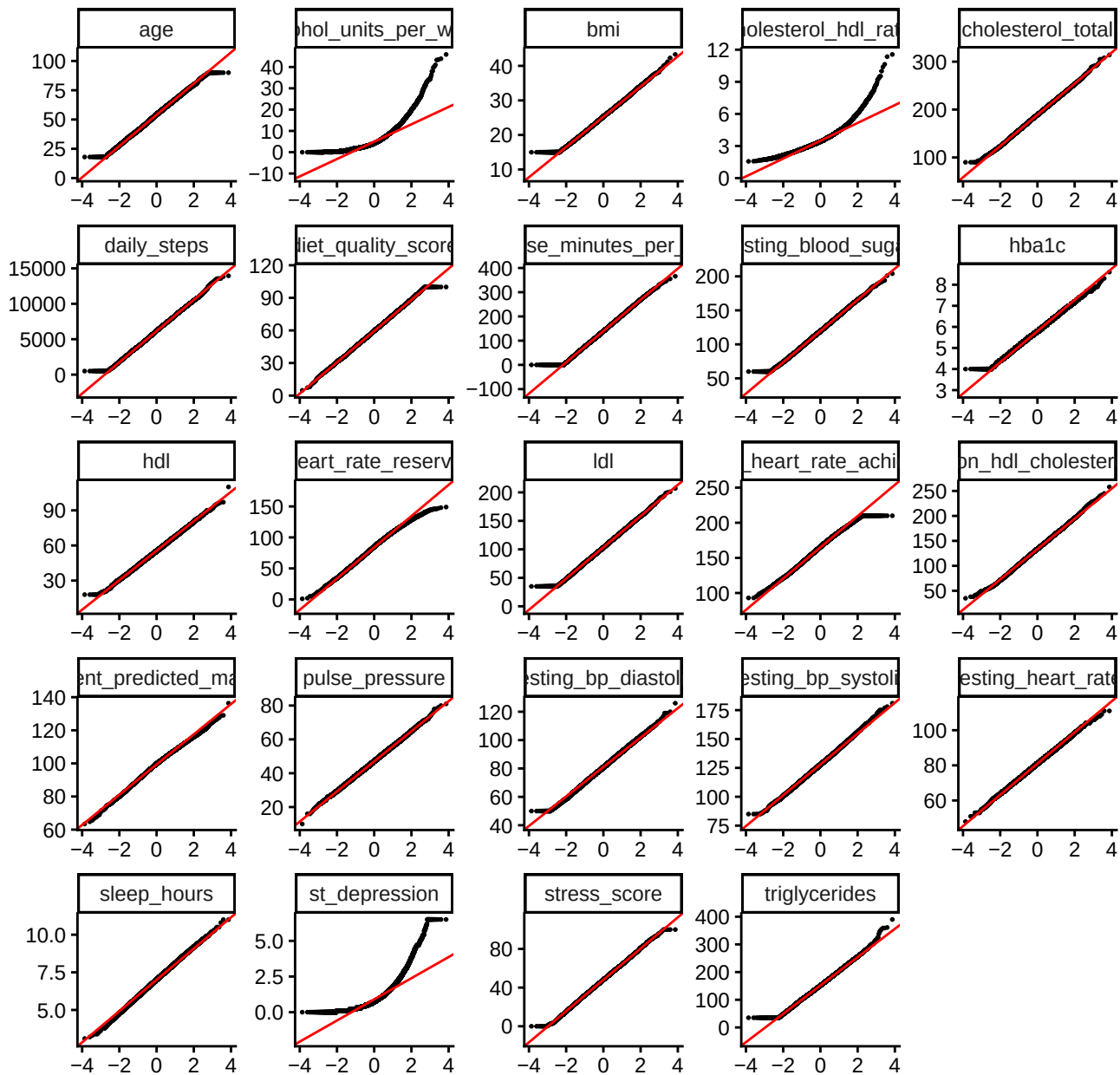
Normal QQ plot of each numerical variable
