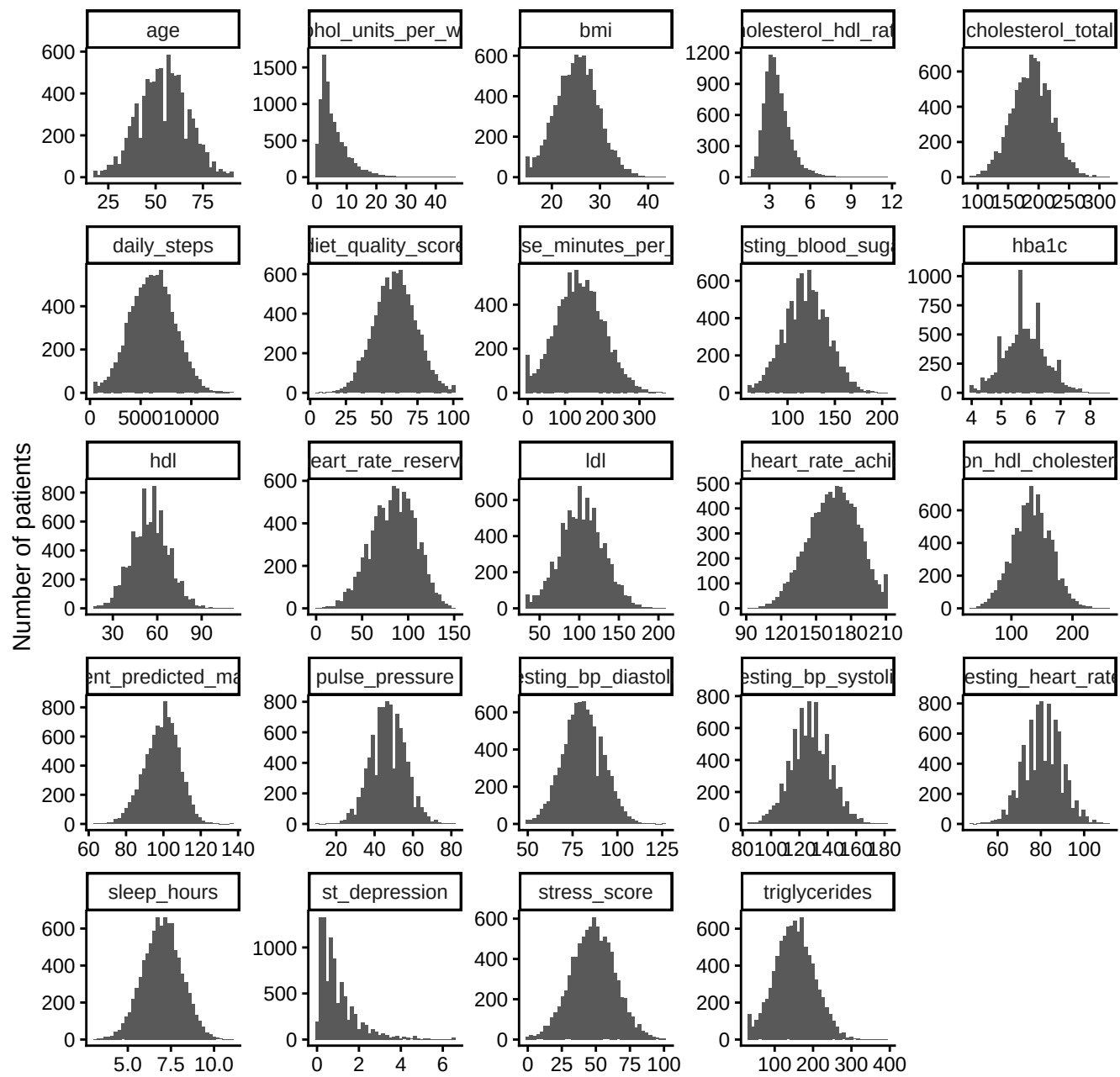
Distribution of each numerical variable
