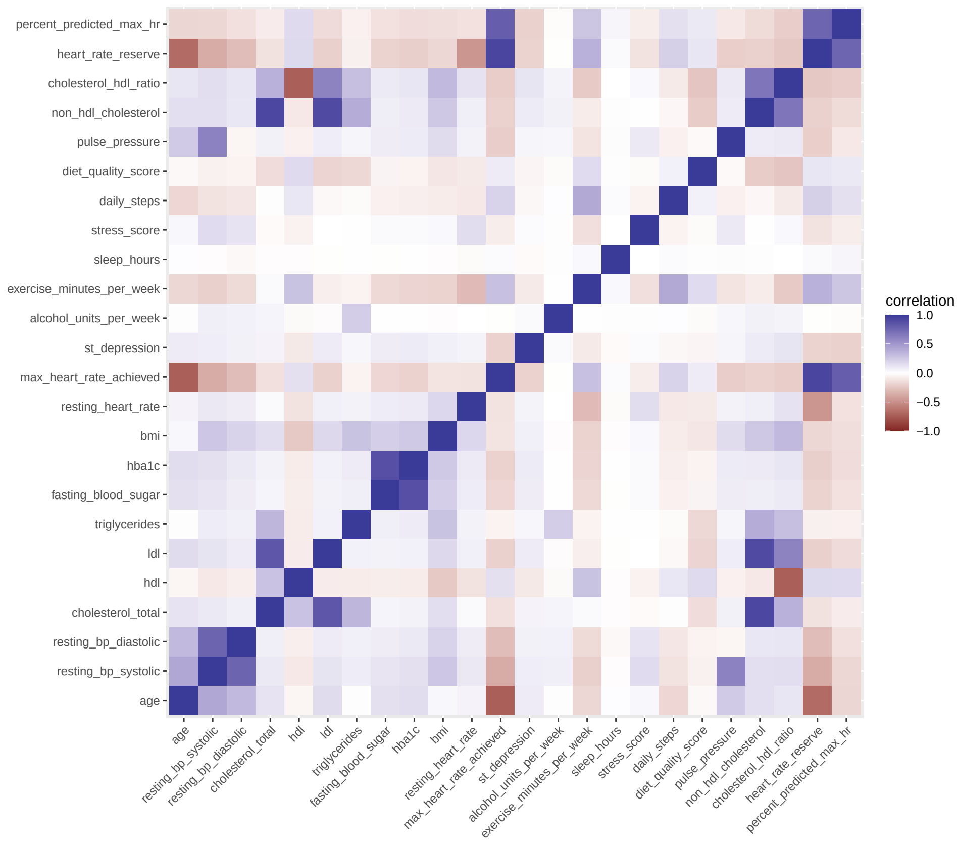
Pearson correlation between the numerical variables
