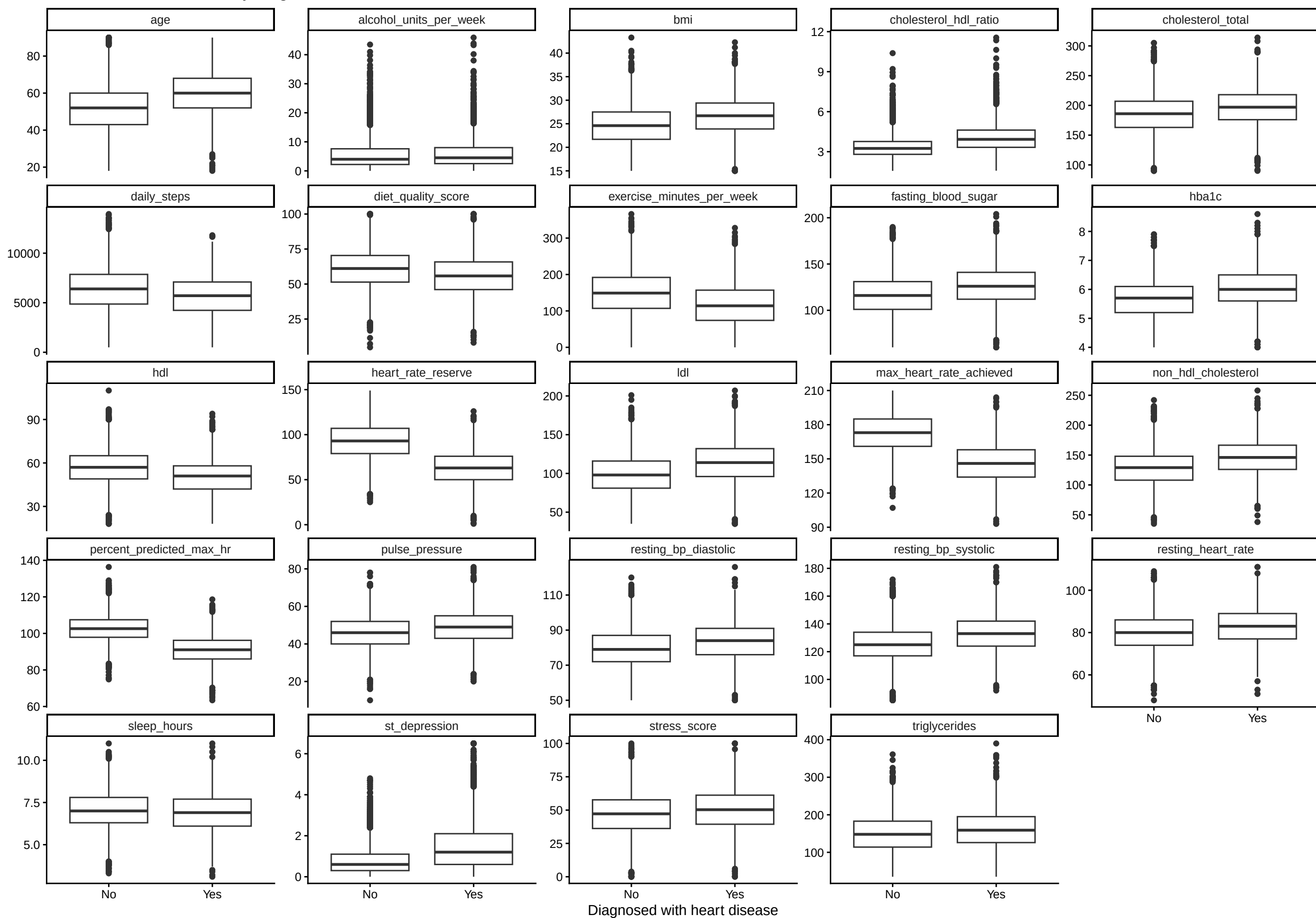
Each numerical variable by diagnosis
