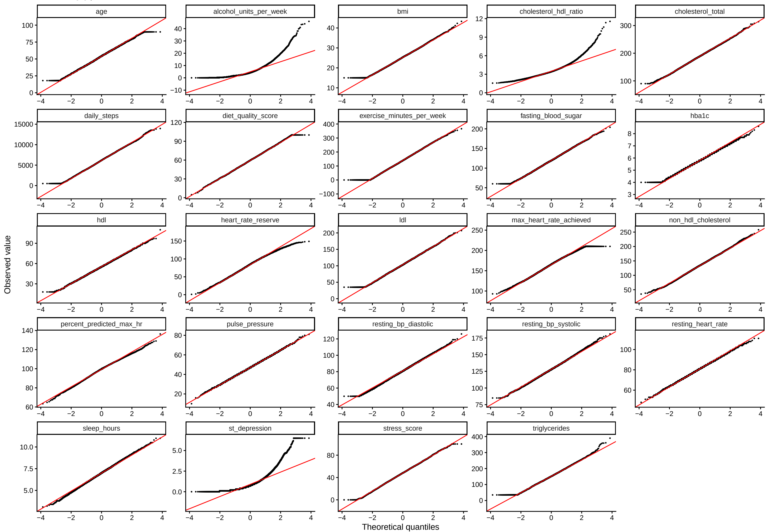
Normal QQ plot of each numerical variable
