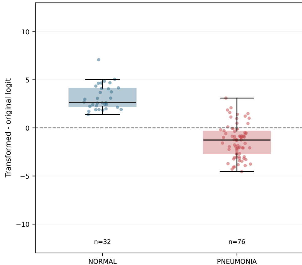
MobileNetV3-Small
