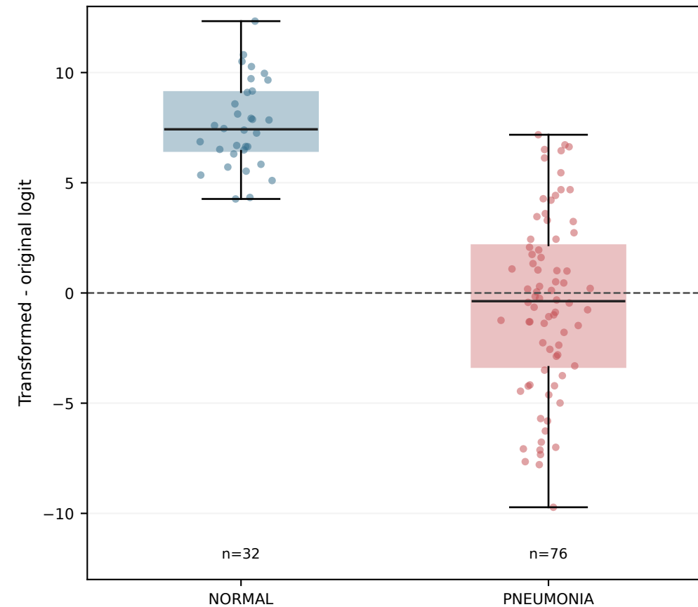
ResNet18
