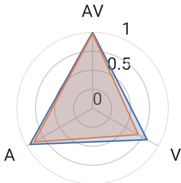
CAV-MAE
