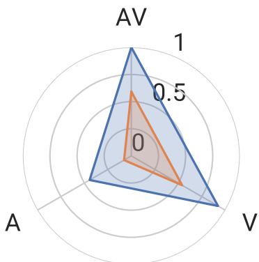
Benchmark
