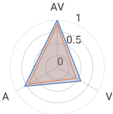
DeepAVFusion
