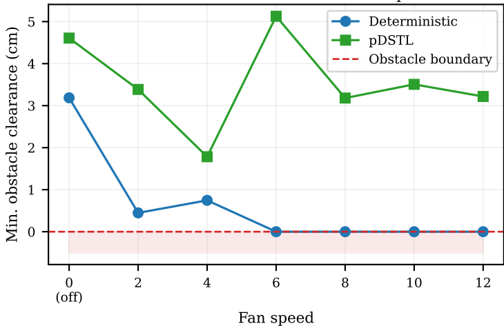
Minimum obstacle clearance vs fan speed
