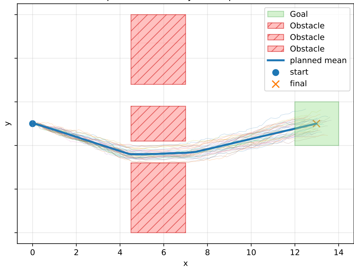
pdSTL uncertainty-aware planner
