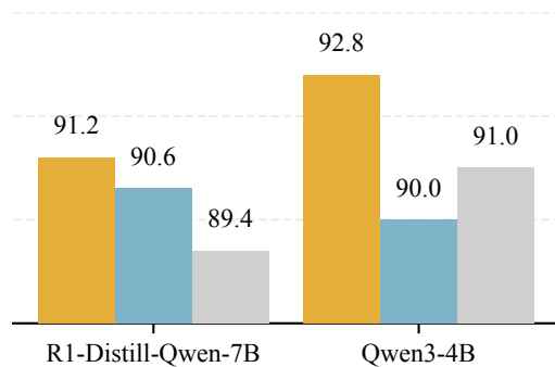
MATH-500
