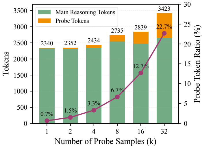
(b) Token Consumption
