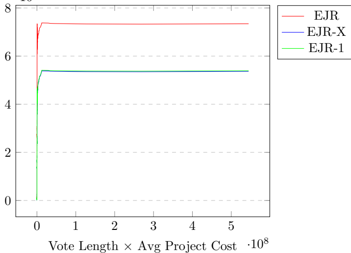
EJR Running Time vs Vote Length \times Avg Project Cost
