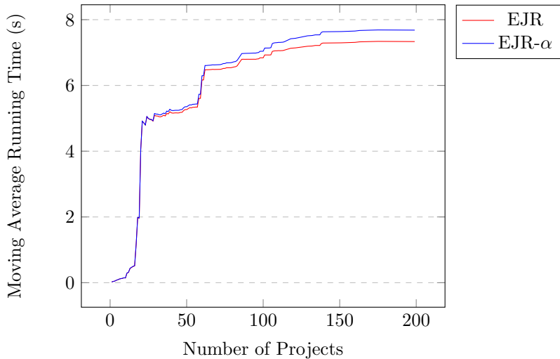
EJR Running Time vs Number of Projects (EJR vs EJ \alpha -exit-early)
