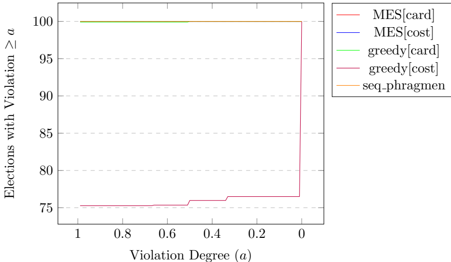
EJR[card] Violation Degree Distribution
