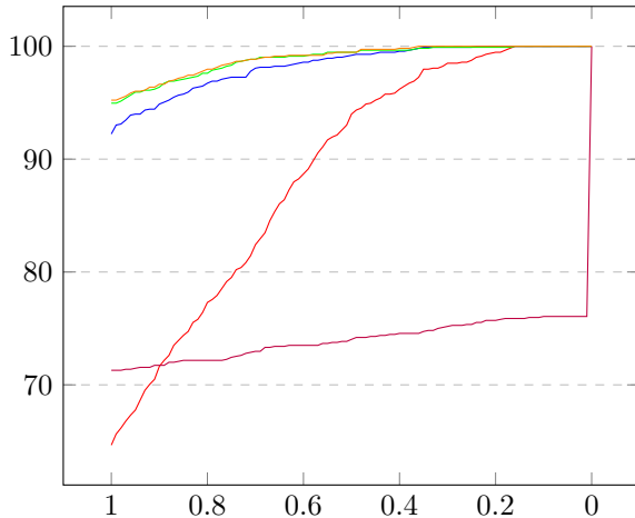
EJR[cost] Violation Degree Distribution
