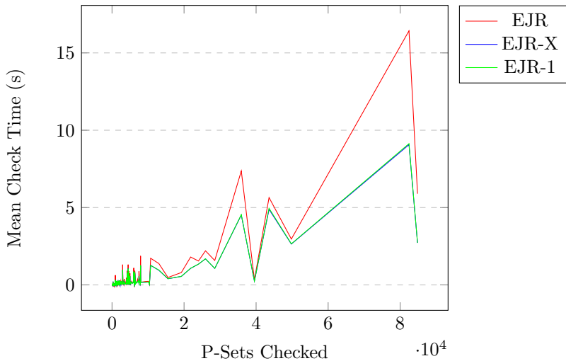
EJR Check Time vs P-Sets Checked
