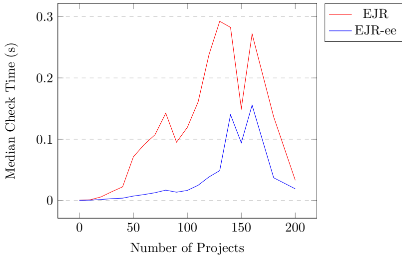
EJR Check Time vs Number of Projects (EJR vs EJR-exit-early)
