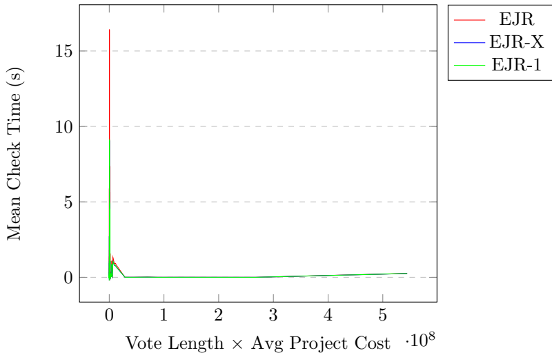
EJR Check Time vs Vote Length \times Avg Project Cost
