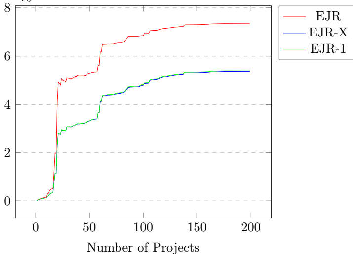
EJR Running Time vs Number of Projects
