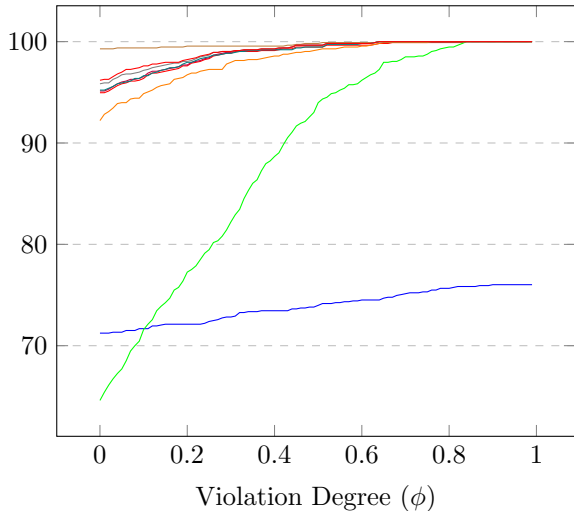
EJR[cost] Violation Degree Distribution
