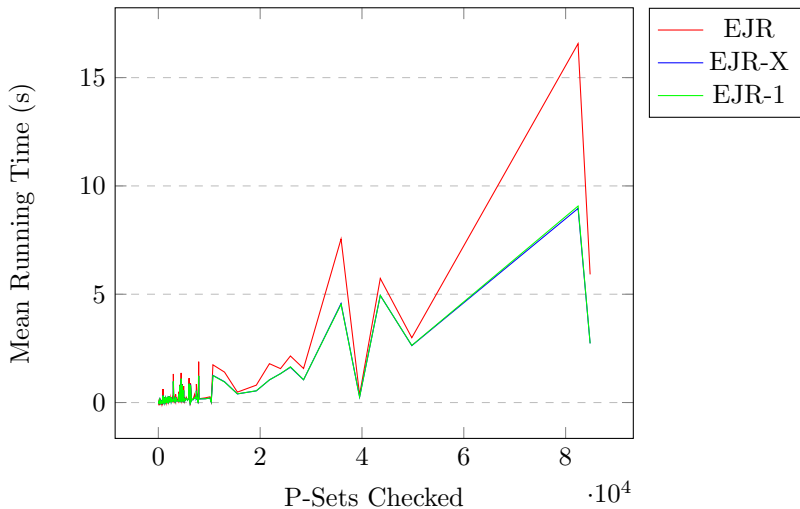
EJR Running Time vs P-Sets Checked (bucket size=5)
