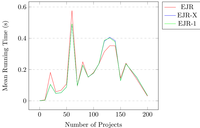
EJR Running Time vs Number of Projects (bucket size=10)
